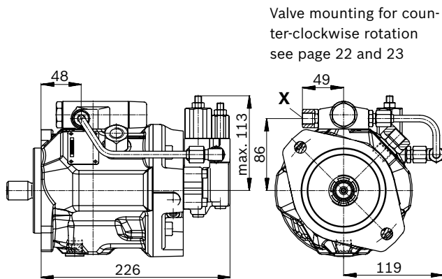
Port plate 11 (61)
