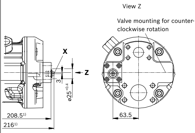
Port plate 11 (61)
